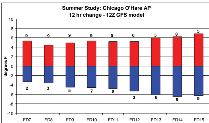
Figure 2. Red and Blue bars represent the ‘average positive’ and ‘average negative’ 12-hour forecast temperature changes for the 12Z GFS. Bold numbers next to each bar represent the number of days that temperature criteria were met for Forecast Days 7 through 15.
