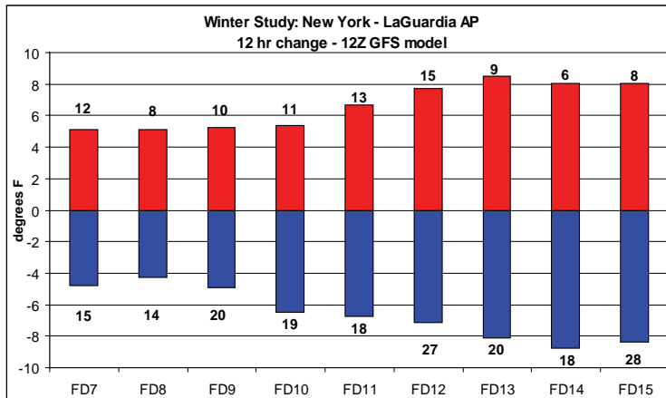
Figure 1. Red and Blue bars represent the ‘average positive’ and ‘average negative’ 12-hour forecast temperature changes for the 12Z GFS. Bold numbers next to each bar represent the number of days that temperature criteria were met for Forecast Days 7 through 15.
